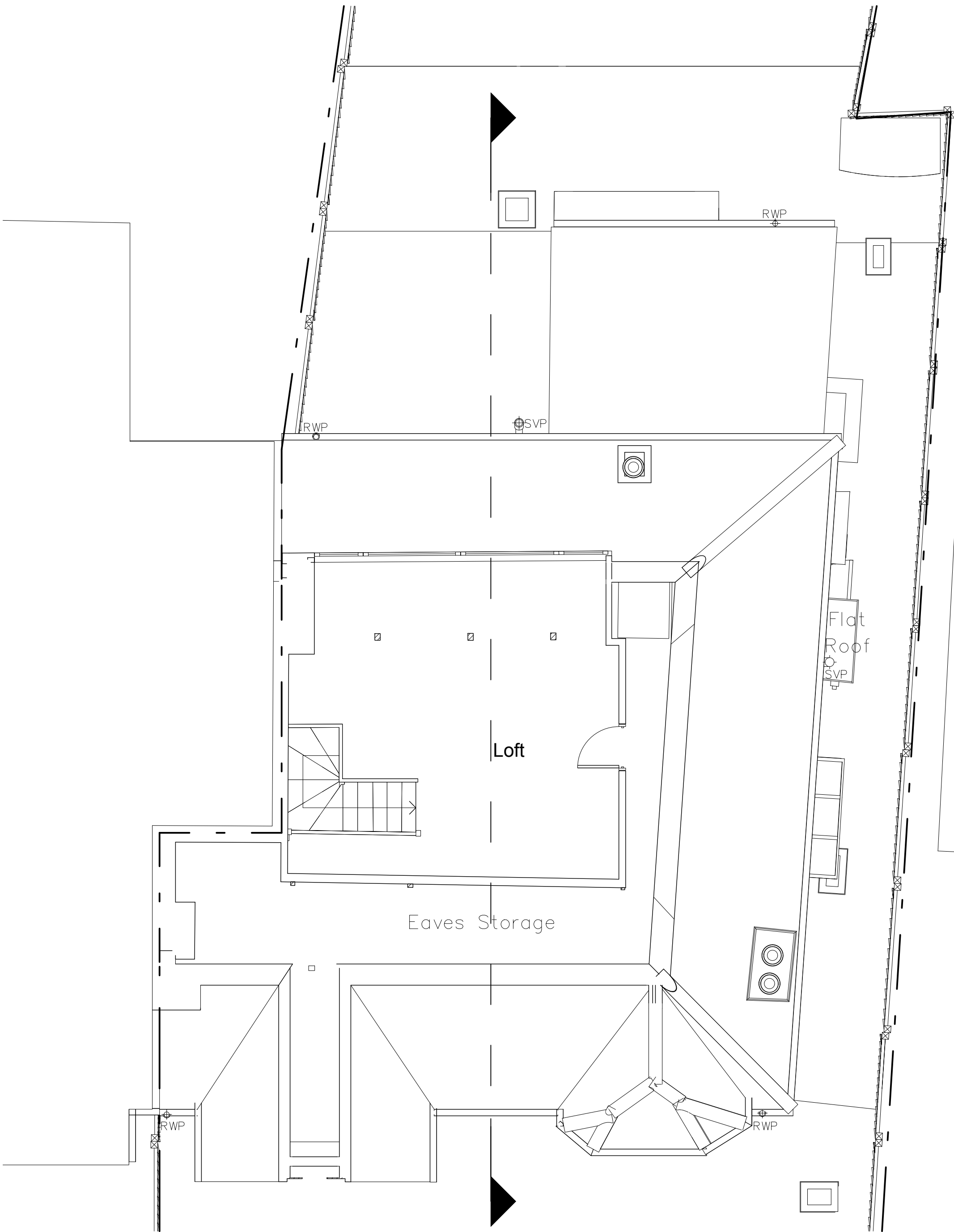
EXISTING LOFT PLAN
